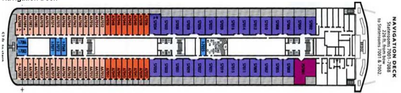
Navigation Deck
